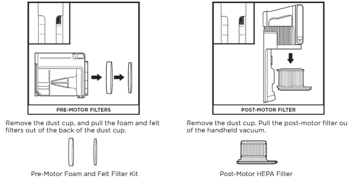
Pre-Motor Foam and Felt Filter Kit Post-Motor HEPA Filter
