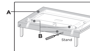
Screws (ST4X25mm)
