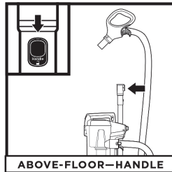
ABOVE-FLOOR—HANDLE Press the Handle Release button to detach the handle from the wand.
