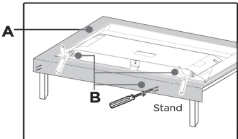
Screws (ST4X25mm)
