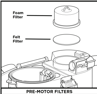
PRE-MOTOR FILTERS
