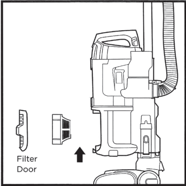
RINSE HEPA FILTER EVERY YEAR Remove dust cup, tilt Filter Door and firmly pull it off. Press tab at top of HEPA Filter and pull out filter. To reinstall, insert HEPA filter into unit and replace the filter door.
