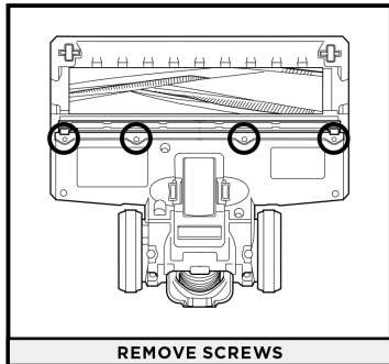
REMOVE SCREWS
